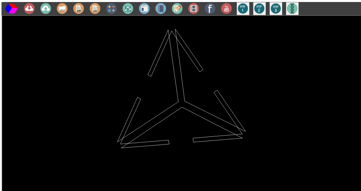
Figure 4: Eulerian Circuit Formation
